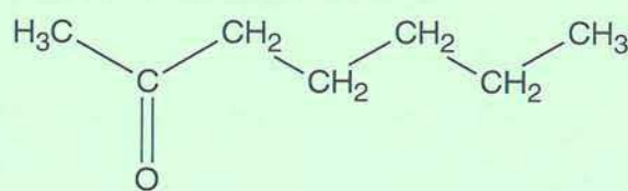
heptan-2-one
